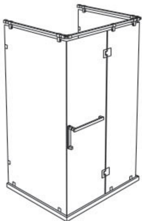
U SHAPE (3 FIX + 1 DOOR)
