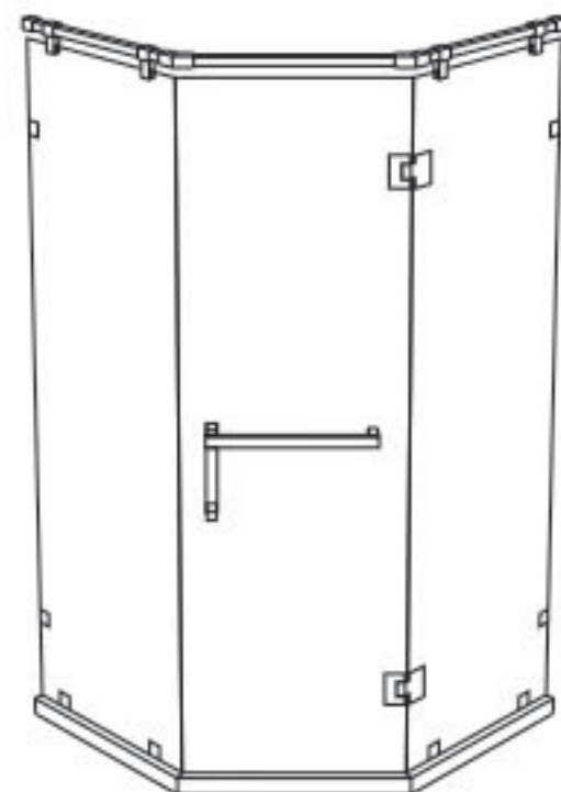
PENTAGON SHAPE (2 FIX + 1 DOOR)
