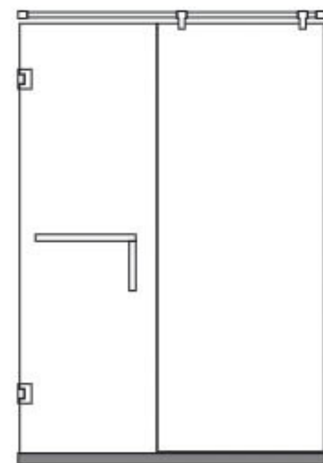
STRAIGHT (1 FIX + 1 DOOR)
